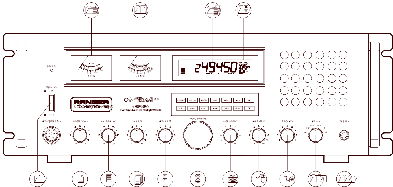
Figure 3-1 Front Panel
